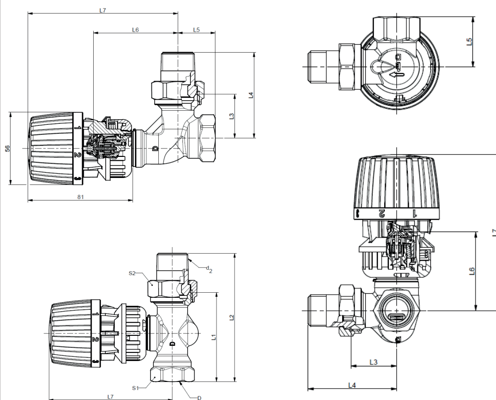
RA-DV DN20 Straight &amp; Angle valve / RA 2990 sensor
